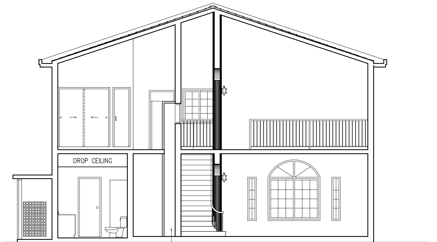
CROSS SECTION
